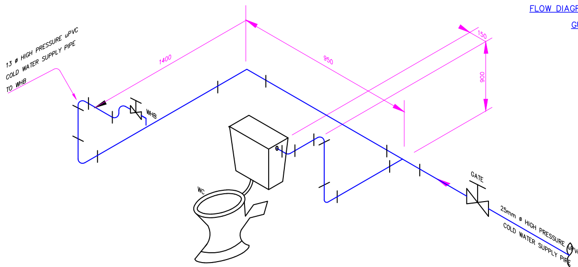
COLD WATER FLOW DIAGRAM
