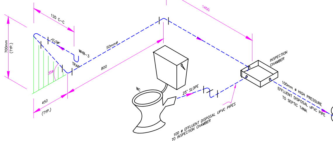
FLOW DIAGRAM OF SEWER SYSTEM GUARD HUT & OFFICE
